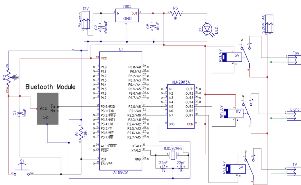
Figure 4. Bluetooth module circuit
