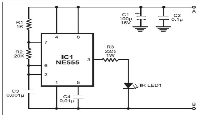
Figure 3. Infra-Red Sensor Circuit
