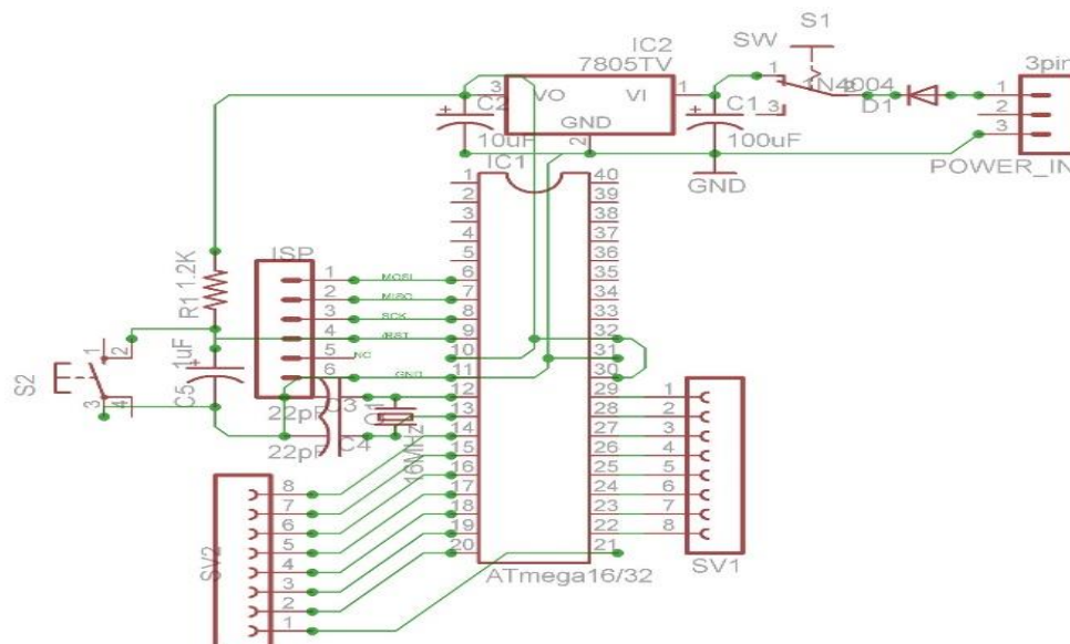
Figure 2. Schematic Of Hardware Circuit Diagrams
